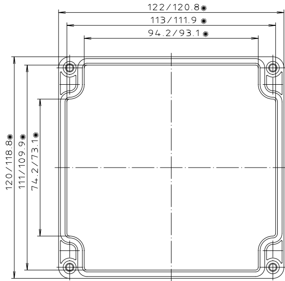
Deckel
